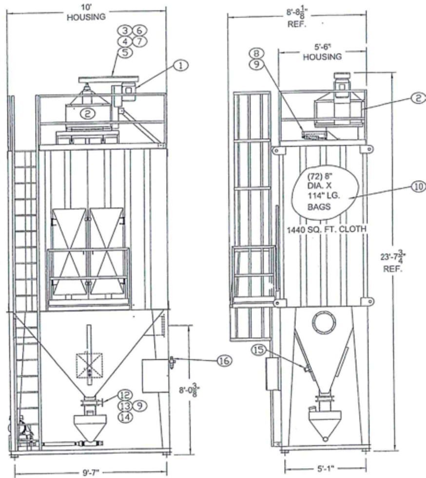
RA-140 DUST COLLECTOR PARTS LIST
