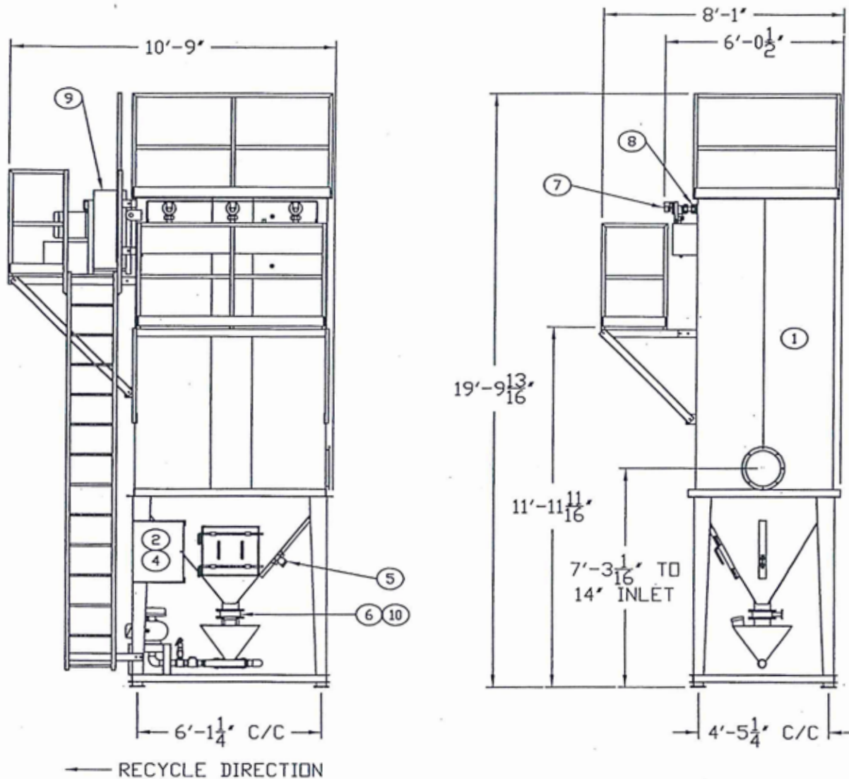
CP-900/ 5250 CARTRIDGE PULSE COLLECTOR WITH OPTIONAL RECYCLE
