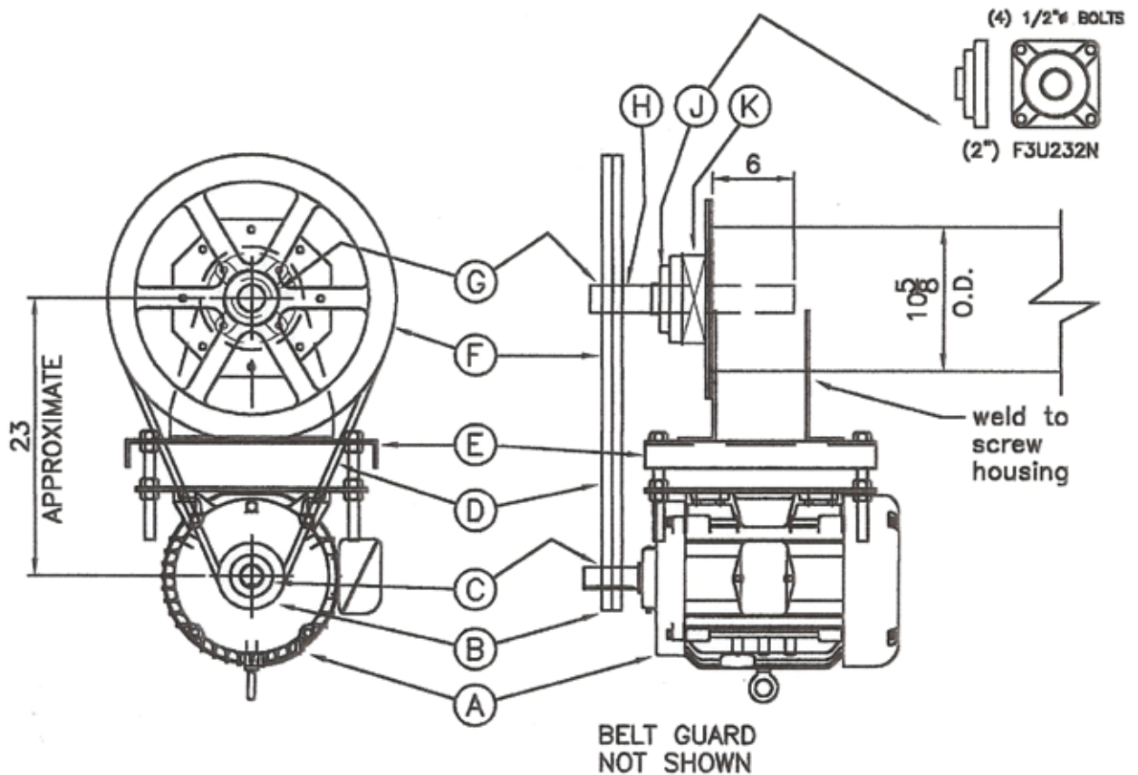
Direct Drive: Shown With Motor Under-Slung
