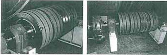
WP-10-900-00200 HUB ASSEMBLY - COMPLETE WITH POWER LOCKING DEVICE; WITHOUT SHAFT
